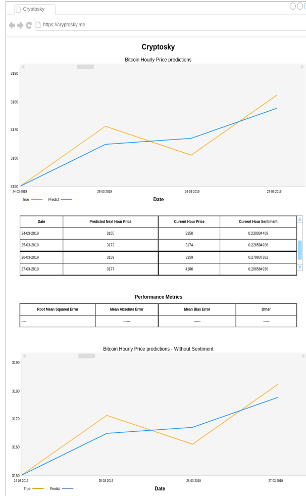
Figure 10: Interface design
